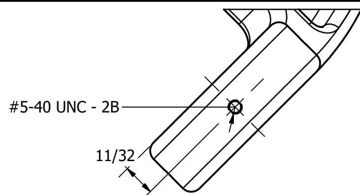
DRILL PRESS BRACKET AUXILIARY VIEW SCALE 1 : 1
