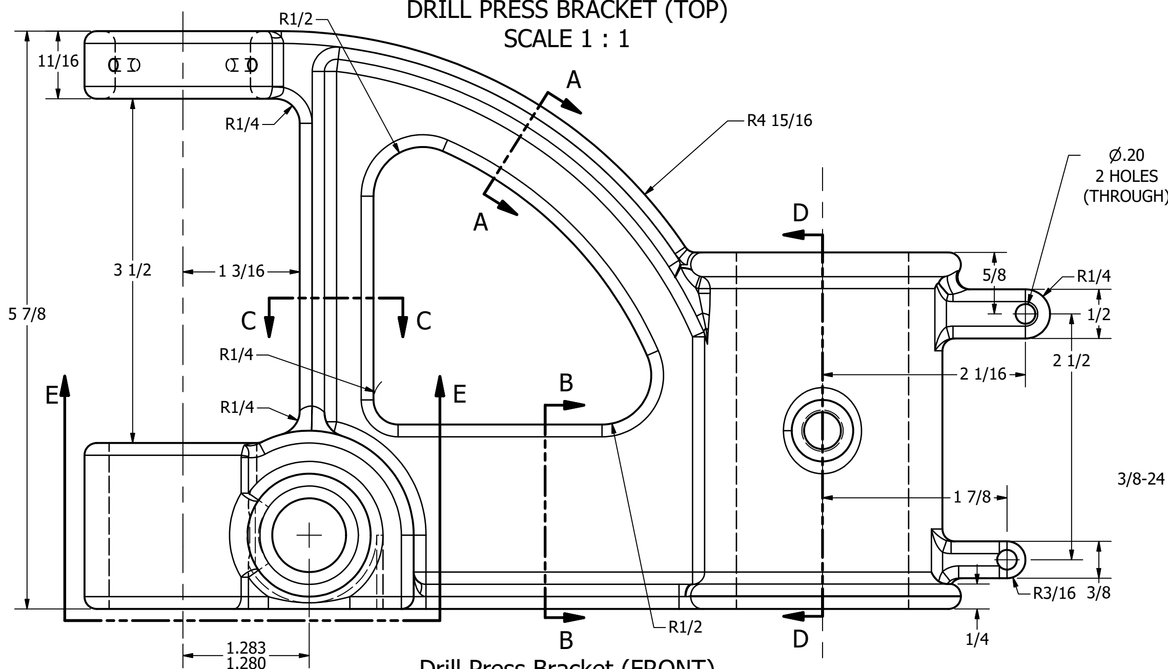
Drill Press Bracket (FRONT) SCALE 1 : 1
