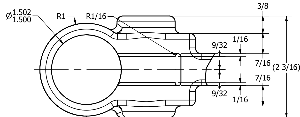
VIEW E-E SCALE 1 : 1
