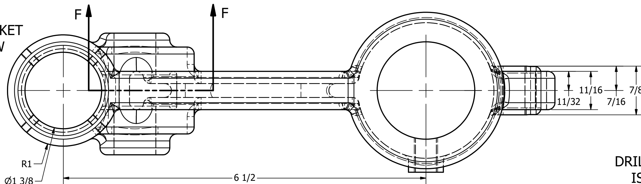
DRILL PRESS BRACKET (TOP) SCALE 1 : 1
