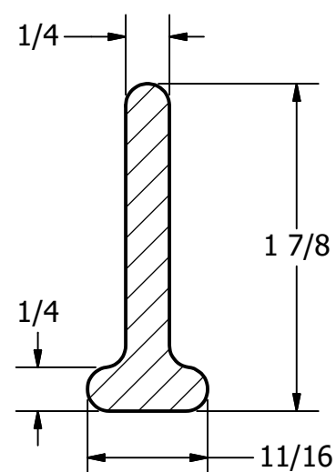
SECTION B-B SCALE 1 : 1
